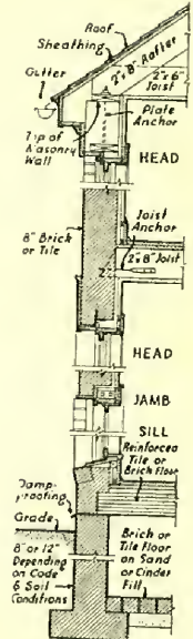
Wall Section
